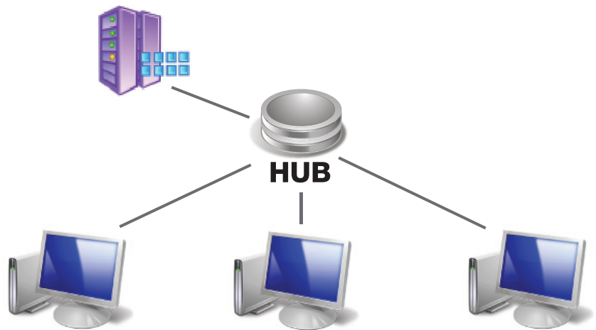
Figure 2: Client/Server Network
